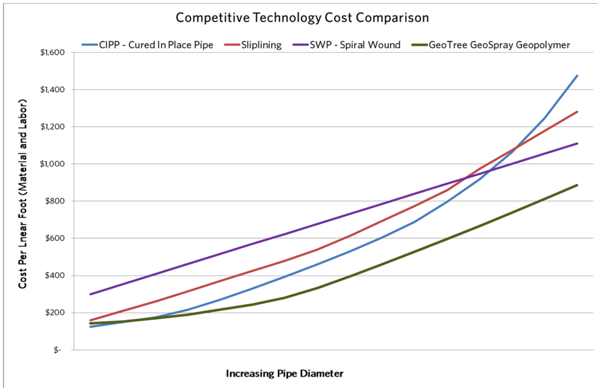
Figure 5: Cost comparison of competitive trenchless technologies
